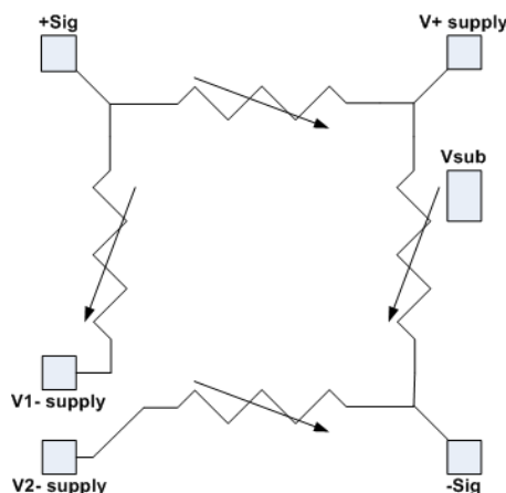
Equivalent Circuit Diagram
