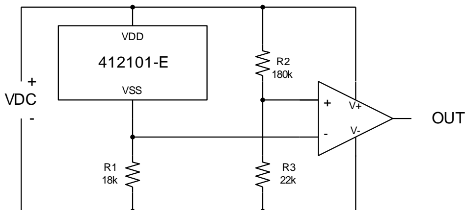
Fig 10 This circuit uses a comparator (or op-amp) to provide a level switching interface for the 412101-E.
